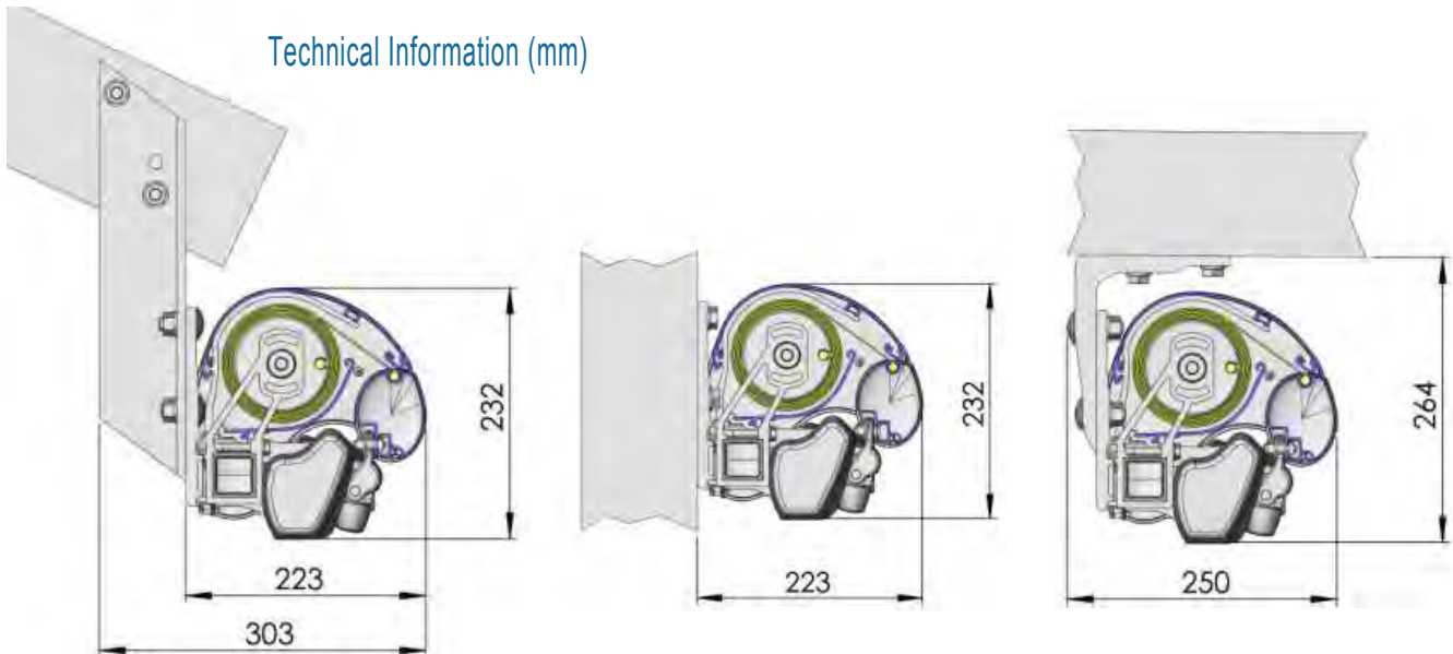
Fitting to the wall wall brackets
