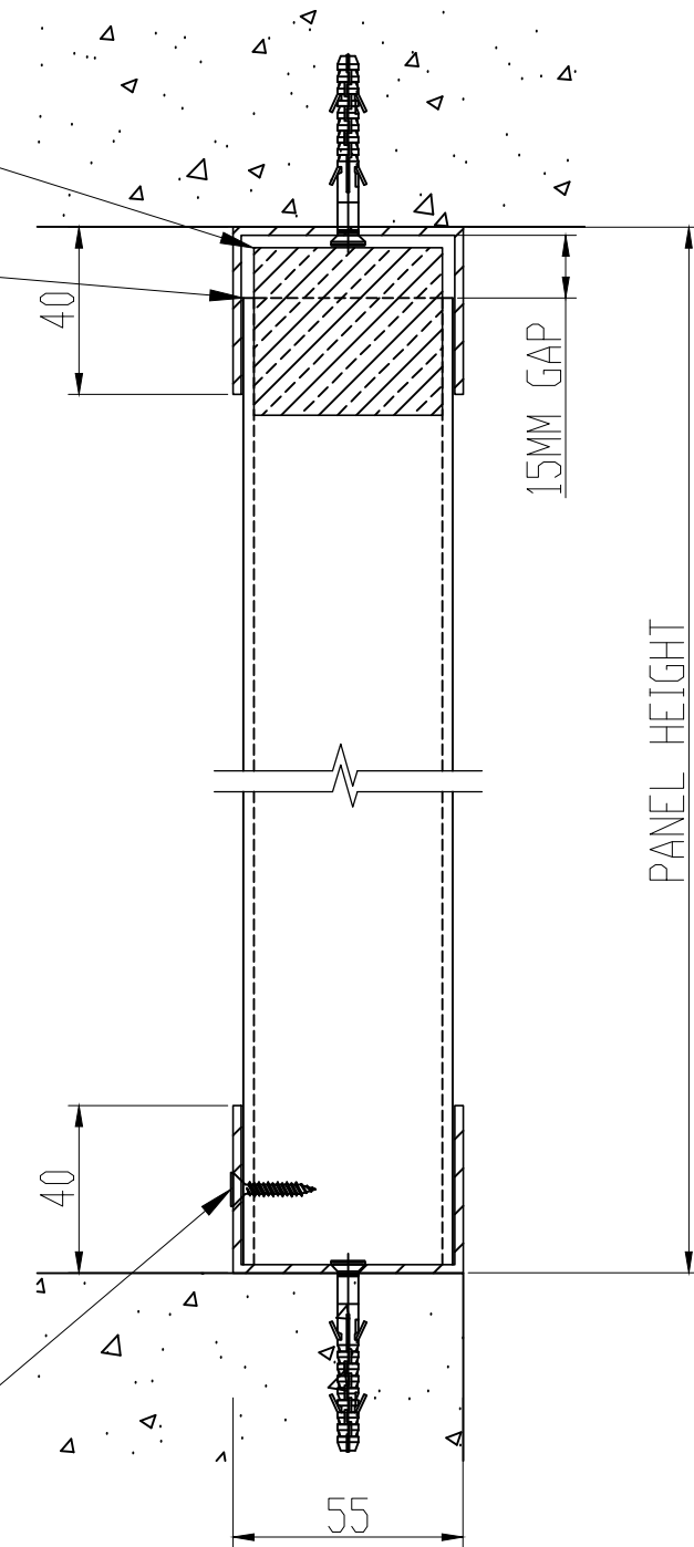
SECTION
