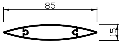
ELIPTICAL LOUVRE BLADE LB 85 EXTRUDED ALUMINIUM
