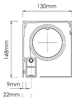
Base bar
