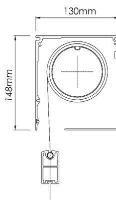
Head box extended bar
