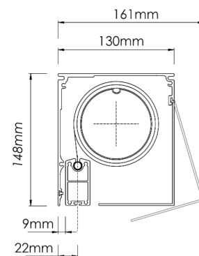
Head box open cover
