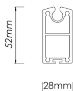
Wall bracket
