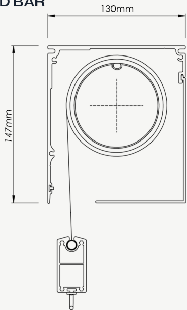
HEAD BOX EXTENDED BAR
