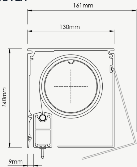
HEAD BOX OPEN COVER
