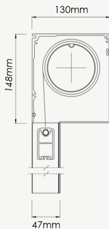
HEAD BOX EXTENDED BAR
