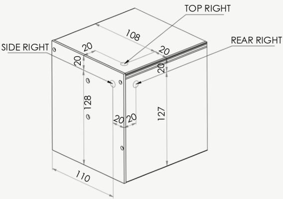
POWER EXIT (RIGHT)
