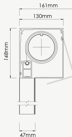
HEAD BOX OPEN COVER
